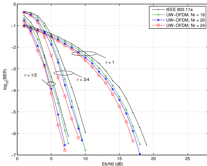
Fig. 7. BER comparison between the novel UW-OFDM approach and the IEEE 802.11a standard for channel B of Fig. 5.
