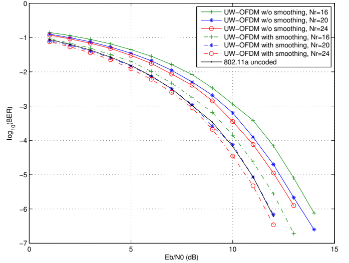
Fig. 4. BER comparison between the novel UW-OFDM approach and the IEEE 802.11a standard in the AWGN channel.
