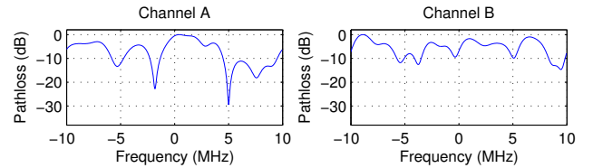
Fig. 5. Frequency responses of the used indoor multipath channel snapshots (equivalent complex baseband presentation as usual).
